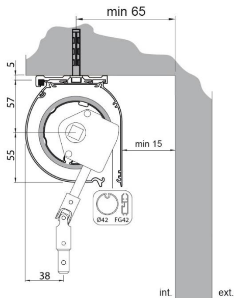
Internal ceiling installation
