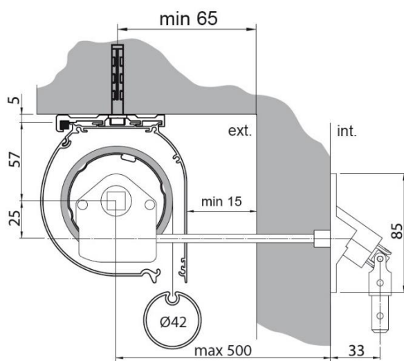
External ceiling installation with wall grommet
